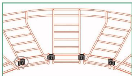
CTW-1-1 Connection Example
