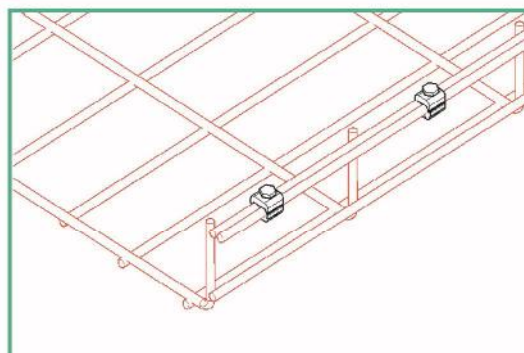
BJ -1 Connection Example
