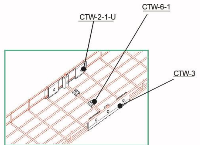
CTW-3 Connection Example
