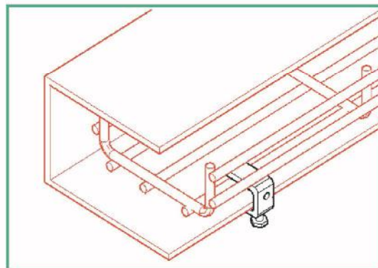
CTW-T4 Connection Example
