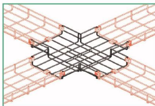
CTW-C10-14 Connection Example
